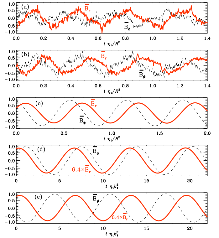
Figure 15. Phase relations of \bar{B}_r (thick red lines) and \bar{B}_\phi (black dashed lines) for Run C1 at (a) 70^\circ and (b) 30^\circ latitude, compared with results of mean-field dynamos of (c) \alpha^2 type and (d), (e) \alpha^2\Omega type, with positive and negative shear, respectively. The amplitudes have been rescaled to unity. Note that only the \alpha^2 dynamo has approximately the phase relation seen in the simulations.
