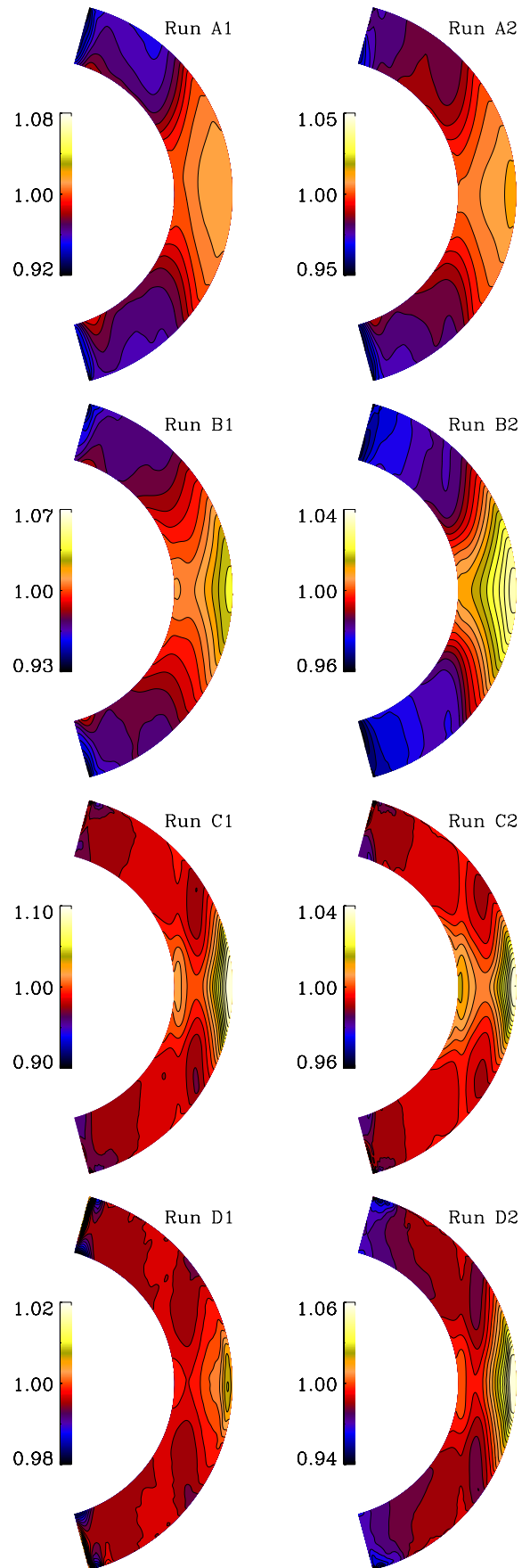
Figure 9. Time averaged mean rotation profiles \bar{\Omega}/\Omega_0 (gray/color scale and line contours) from Sets A, B, C, and D.
