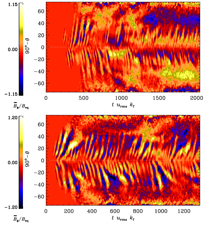
Figure 5. Same as Figure 4, but for Runs B1 (top) and B2 (bottom).
